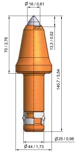
BTK99 B40 / 3-LSK
