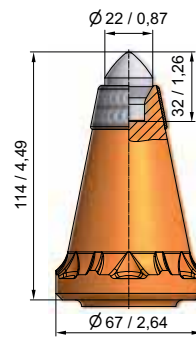
BSR206 BS43H - 73.67114P
