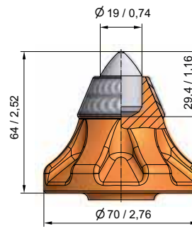
BGS84 B47GK19 / 70-P
