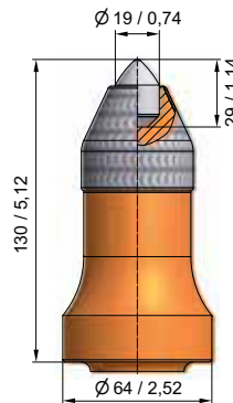
BKR24 BKR19LK130 64P
