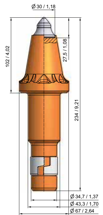
BSR181 BS43H - 69.67102A
