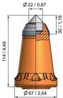
BSR178 BS43H - 22.67114P
