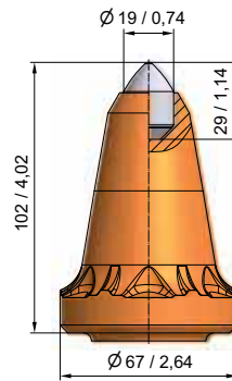
BSR204 BS43H - 19.67102H
