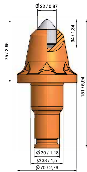
BK17 B47K22 / 70-F
