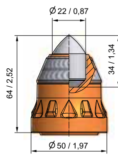
BKS156 / P BS38W-22.5064P
