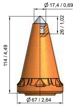
BSR191 BS43H - 70.67114A
