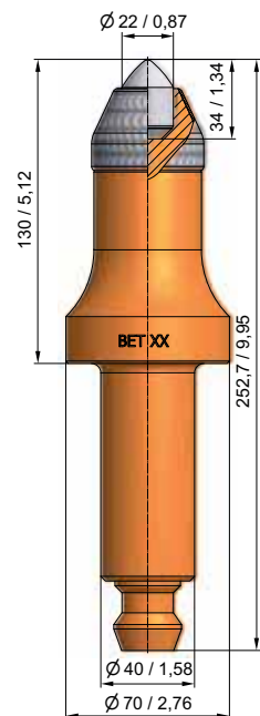
BKR28 BG40X - 22.70130P
